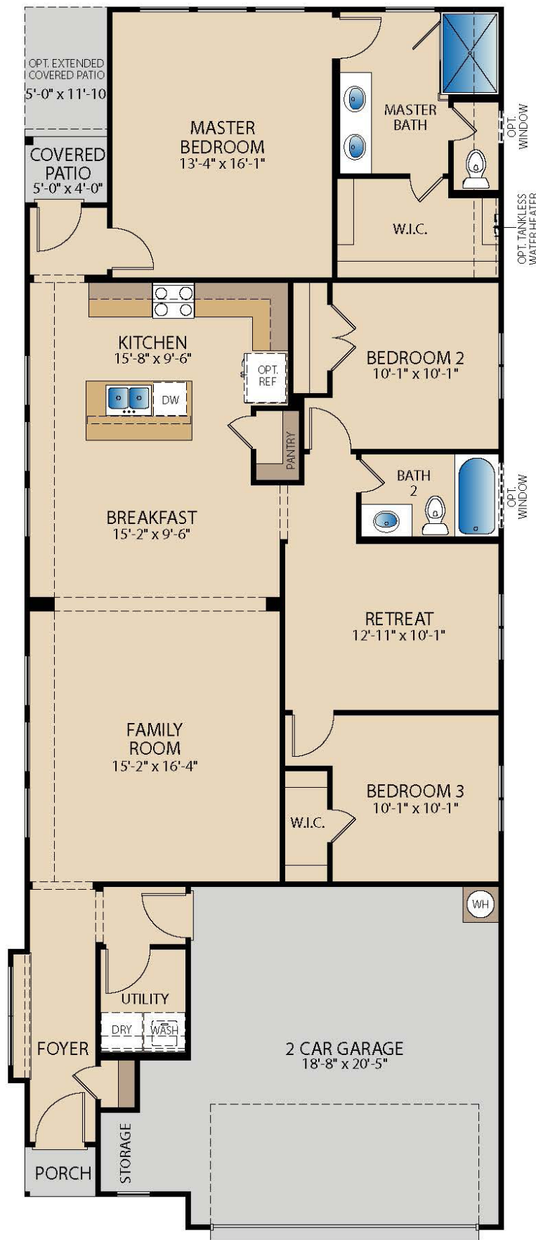
FIRST FLOOR
