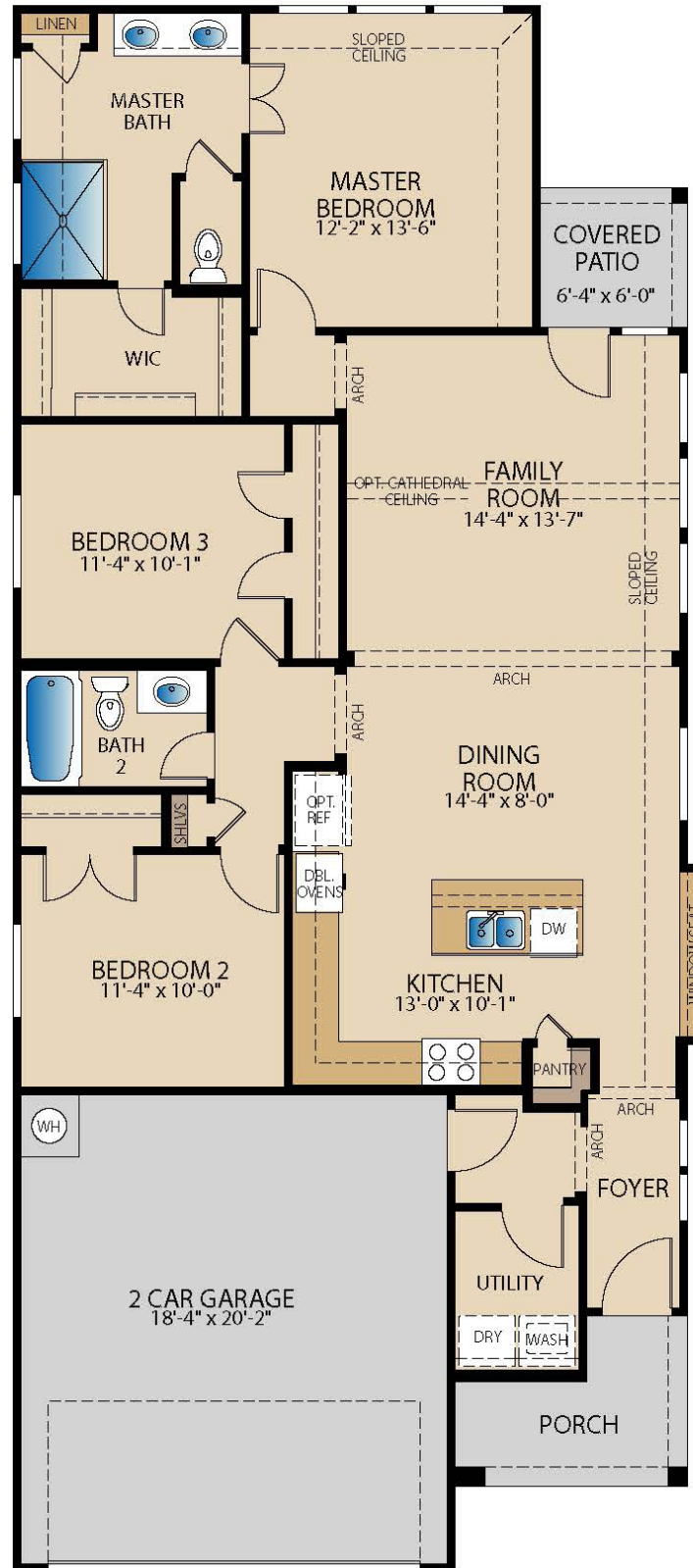
FIRST FLOOR
