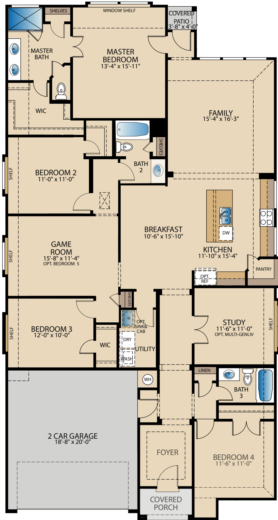
FLOOR PLAN
