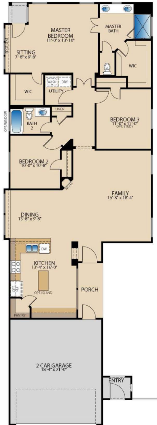
FLOOR PLAN
